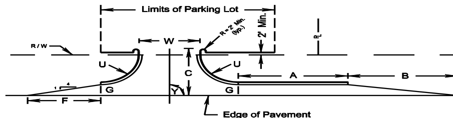
FIGURE 4- 9 COMMERCIAL ENTRANCE DESIGNS ALONG HIGHWAYS WITH SHOULDERS
