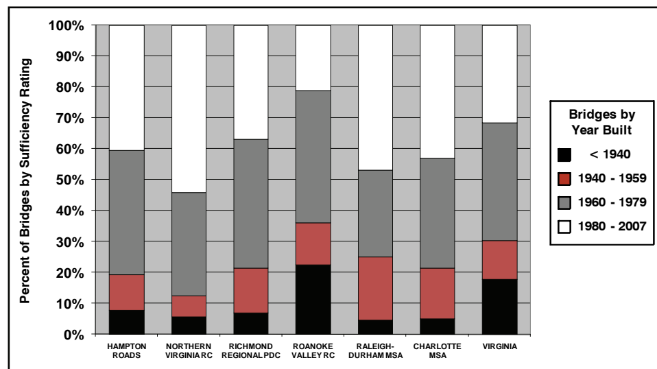
FIGURE 4 – Bridges by Year Built in Selected Areas
