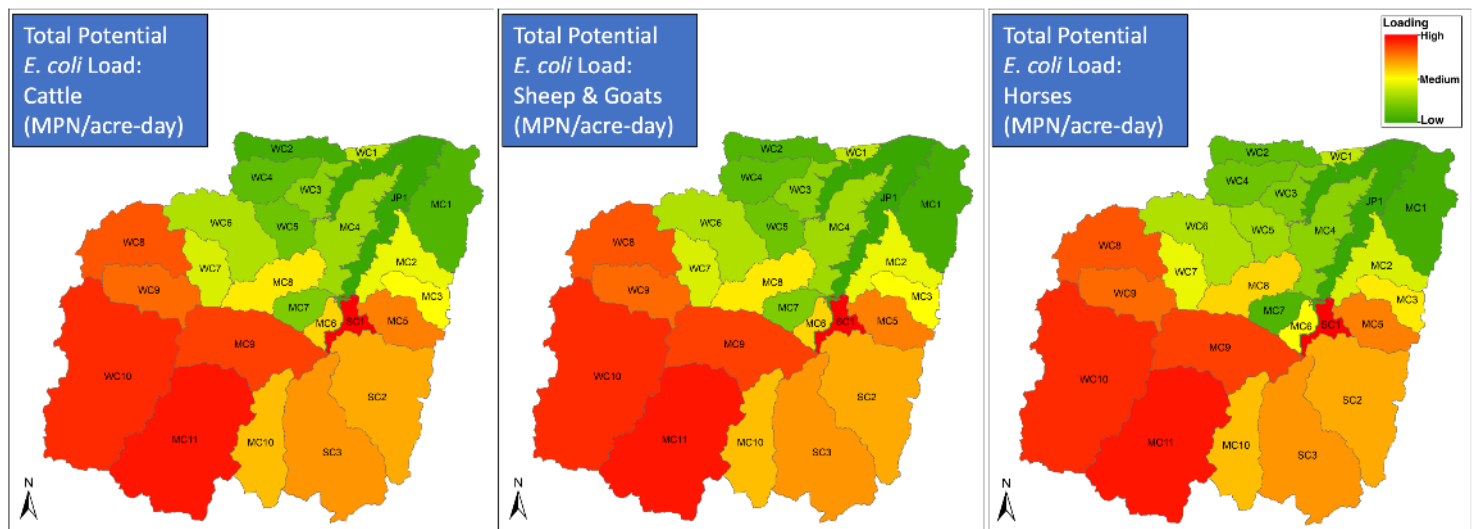
Figure 5-23 Relative severity of E. coli loads from cattle, sheep & goats, and horses, by subwatershed
