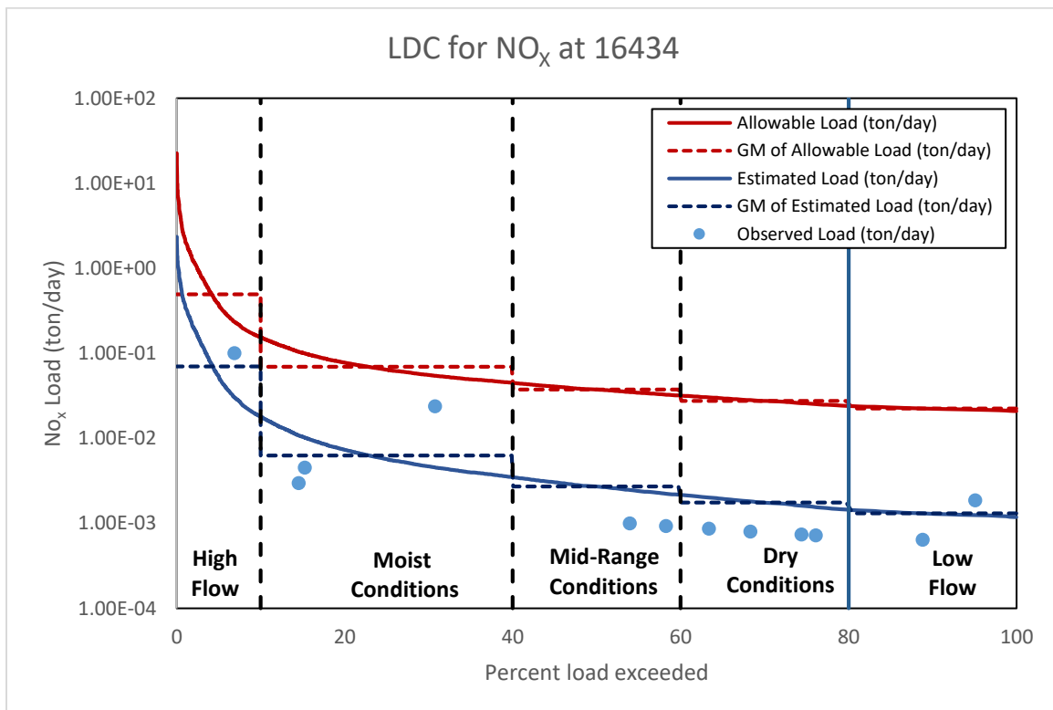
Figure G-16 LDC for NO x at surface water quality monitoring station 16434
