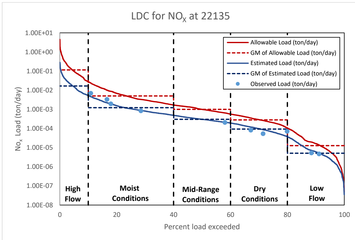
Figure G-6 LDC for NO x at surface water quality monitoring station 22135
