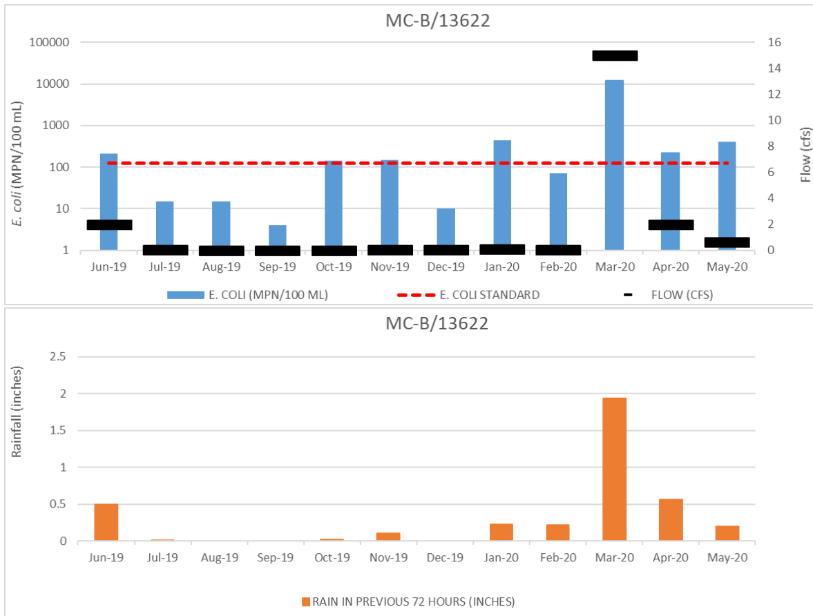
Figure E-5 Hydrology and E. coli Parameters, Mountain Creek at FM 157 (13622)
