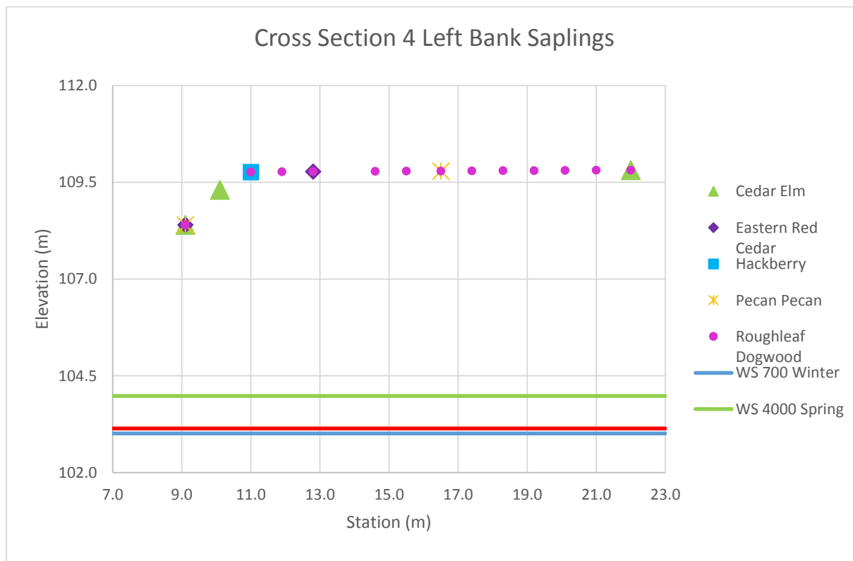
Figure 42. 080444 – Cross-section 4 – Left Bank – Seedlings – Location along cross-section.
