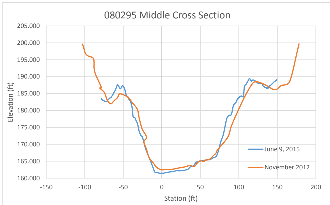
Figure 58. 080295 middle (xs2) cross-section comparison (elevations in feet above NAVD88).
