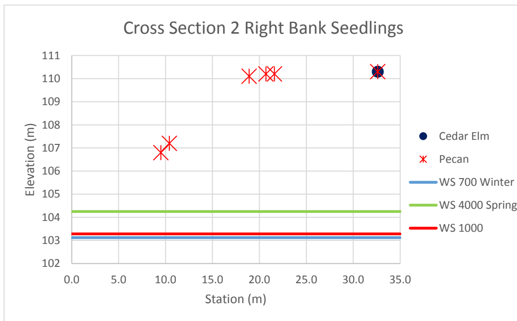
Figure 40. 080444 – Cross-section 2 – Right Bank – Seedlings – Location along cross-section.
