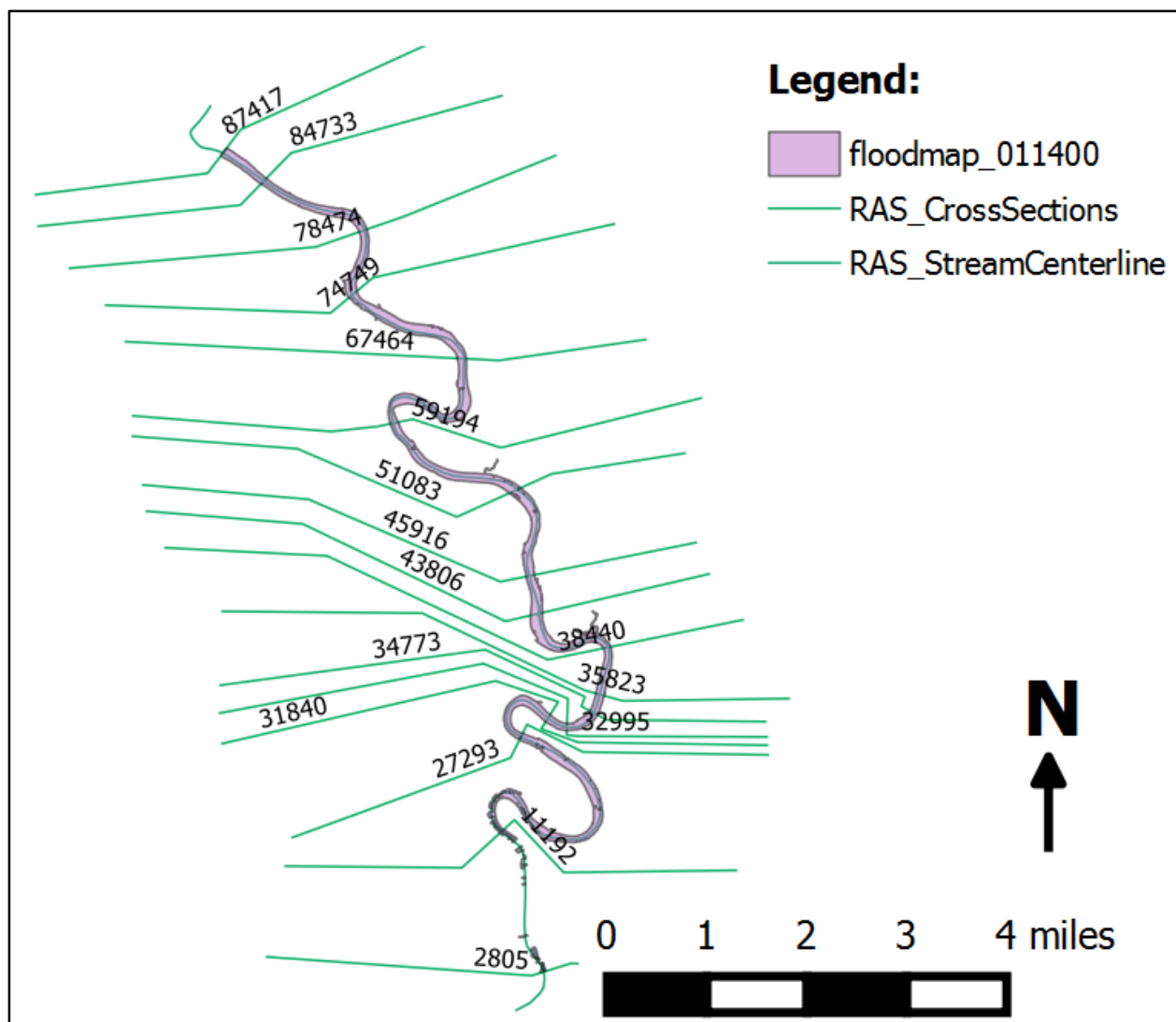
Figure 93. 080075 – HEC-RAS cross-section locations.
