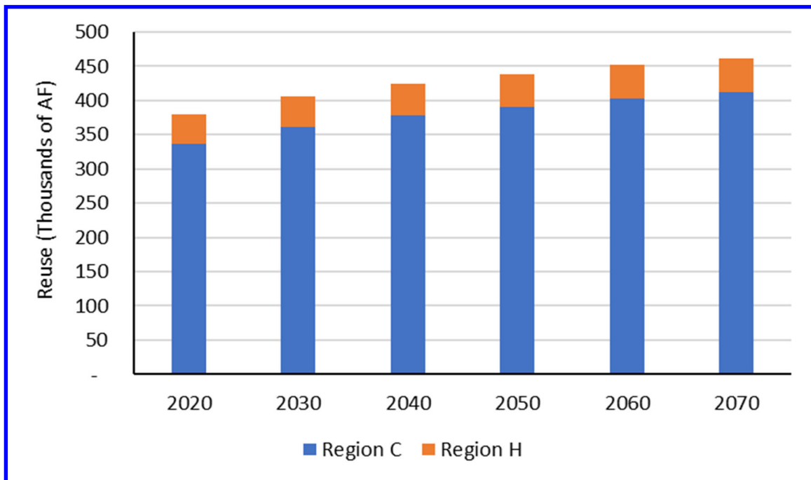
Fig. 4a. 2020 to 2070 Indirect/Direct Reuse Estimates for Regions C and H
