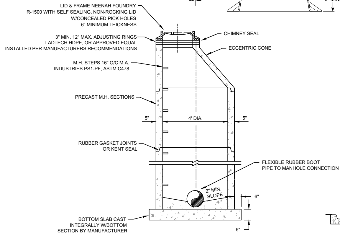
NO SCALE STANDARD PRECAST SANITARY MANHOLE
