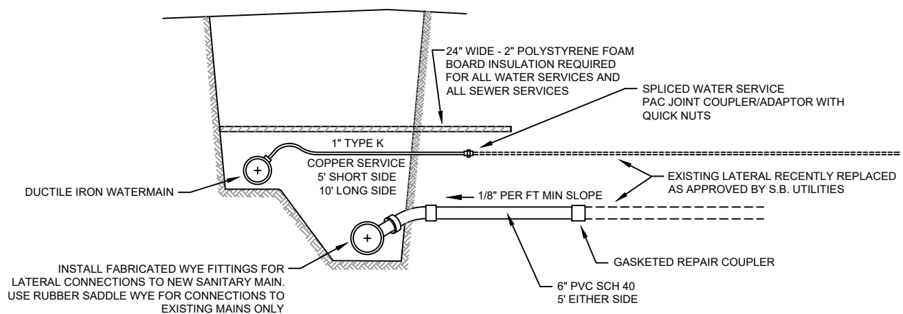
NO SCALE TYPICAL SPLICED SANITARY & WATER SERVICE CONNECTION
