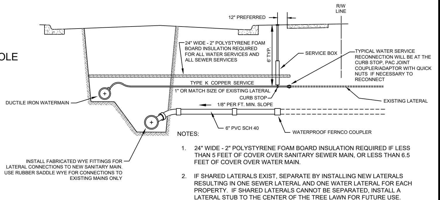
NO SCALE TYPICAL NEW SANITARY & WATER SERVICE CONNECTION
