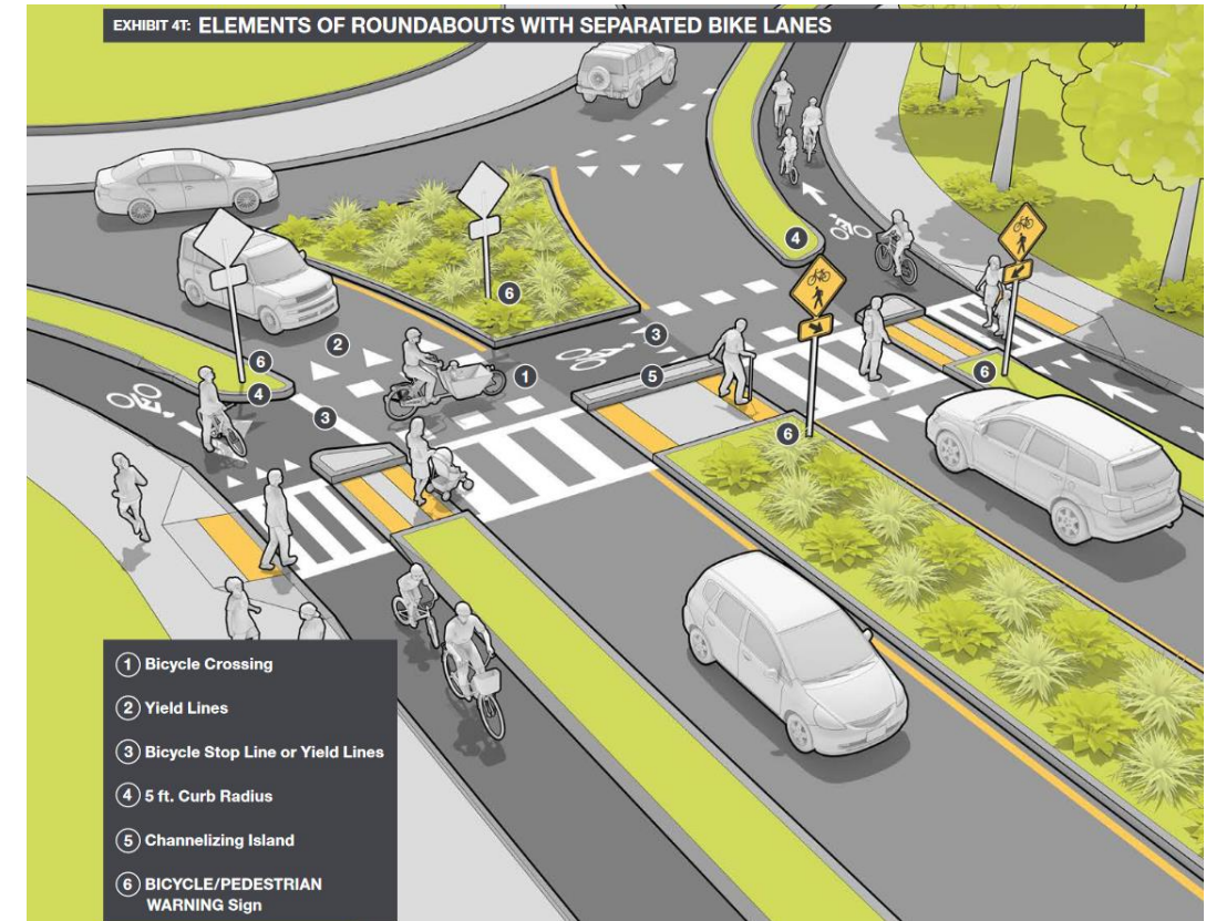
Massachusetts DOT diagram showing guidance for roundabouts with protected (separated) bike lanes and crossings based on best practices from the Netherlands ( https://www.mass.gov/doc/chapter-4-intersection-design-0/download ).
