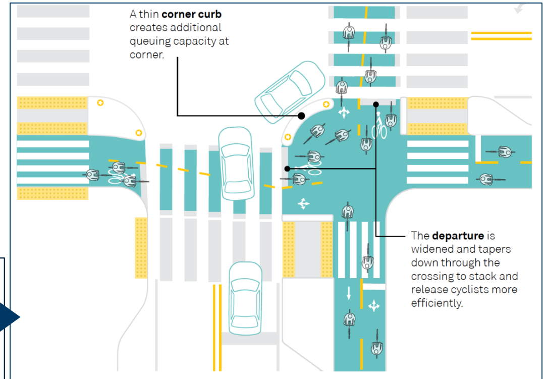
Alternative design for two-way bicycle traffic on one side of the road. Source: NACTO, "Don't Give Up at the Intersection" Variations | National Association of City Transportation Officials ( nacto.org )
