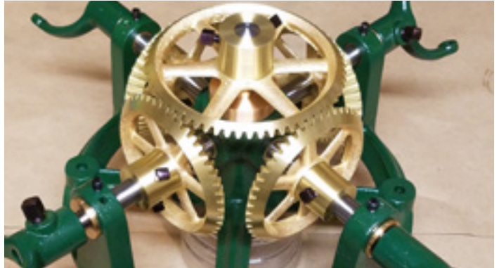
Clock four-way mechanism after restoration.
