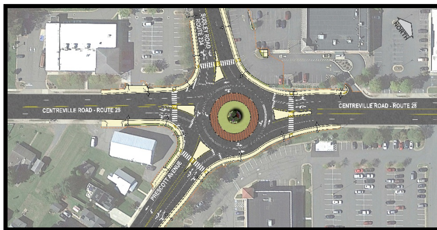
PROPOSED ROUNDABOUT – PLAN VIEW
