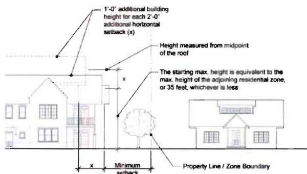
Figure 3.1 Vertical Height Transition
