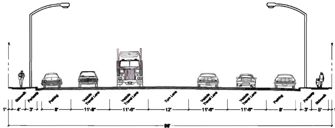
Existing Conditions 400 North Cross Section (approx. 350 East)
