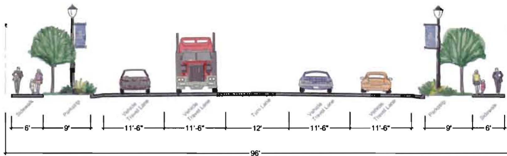
Alternative Road Design (1) 400 North Cross Section (approx. 350 East)
