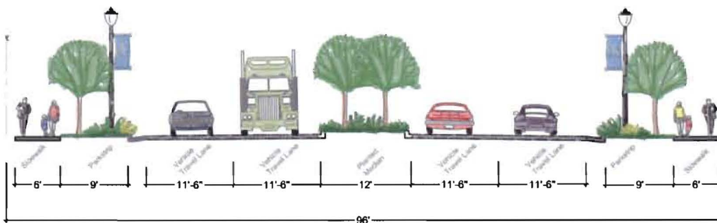
Alternative Road Design (2) 400 North Cross Section (approx. 350 East)
