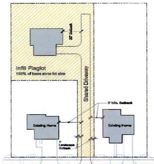
Figure 2.3 Flag Lot
