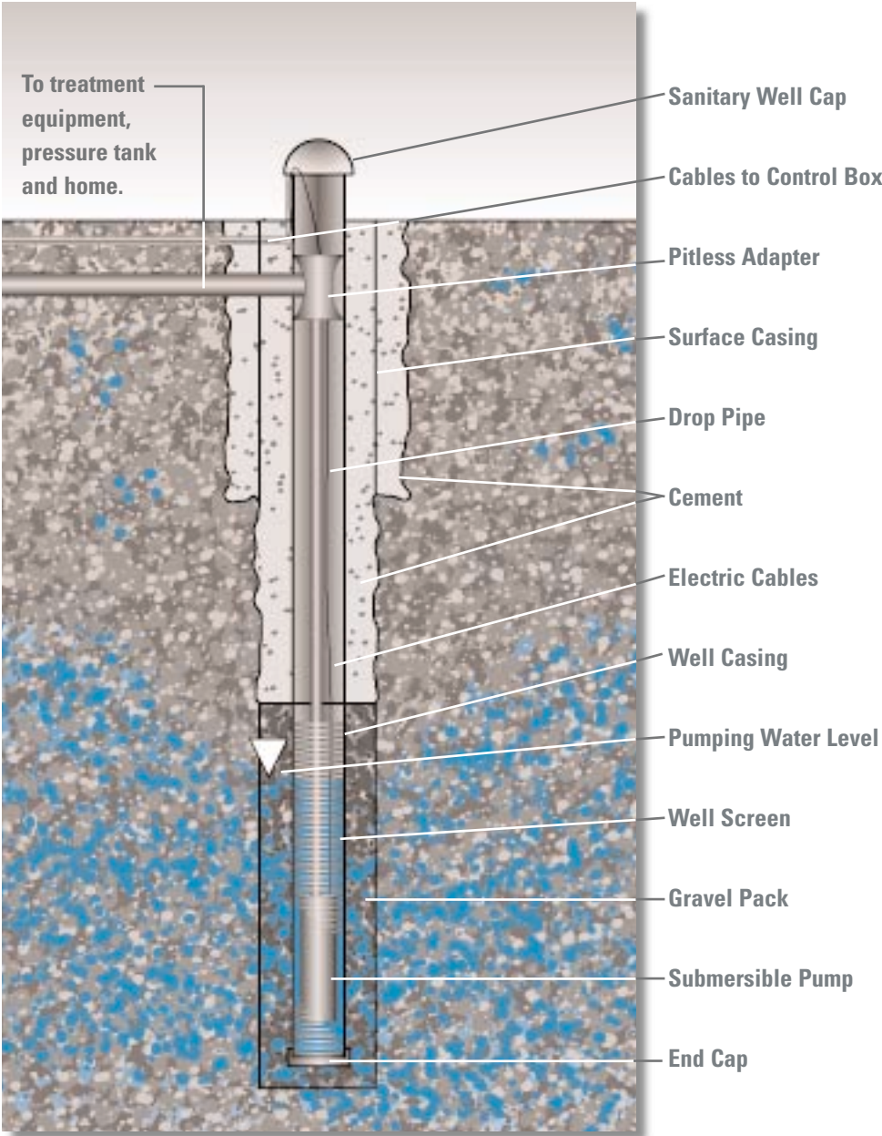
Typical Water Well Construction
