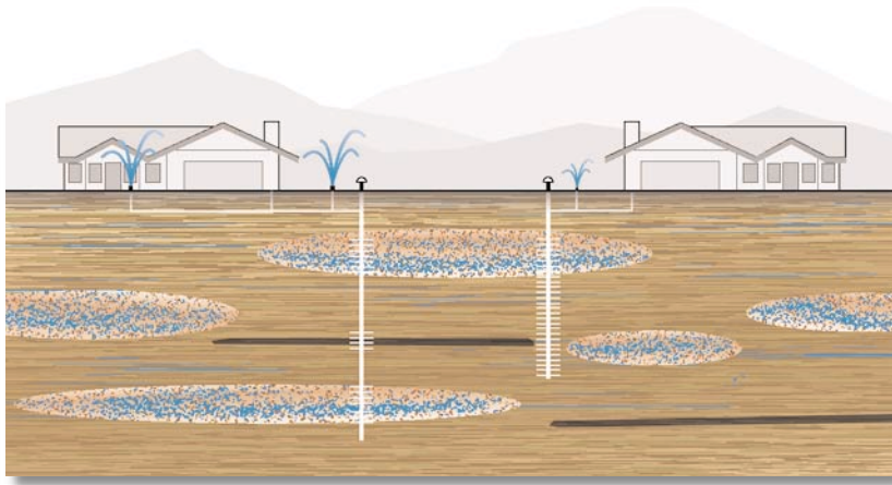
Bedrock Shale and Sandstone Aquifer
