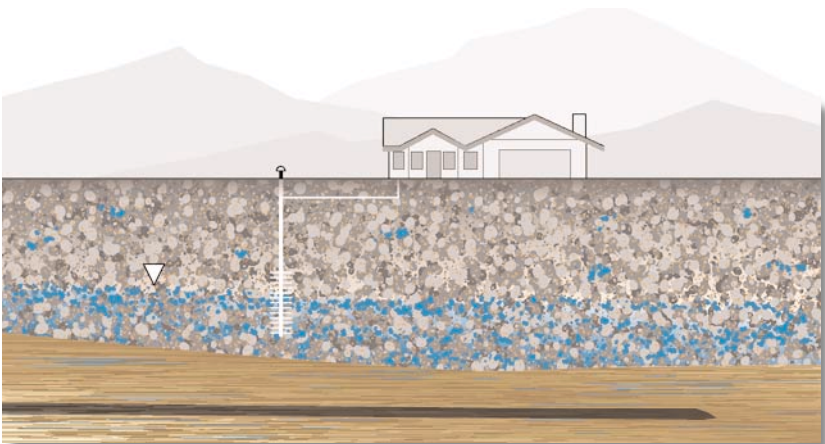
Florida Mesa Aquifer
