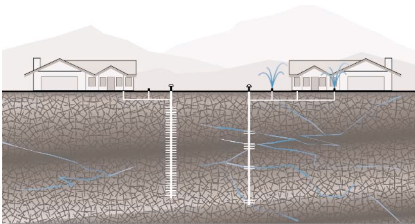
Crystalline Fractured Aquifer
