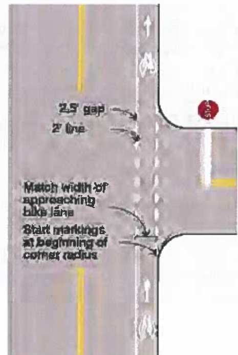
Figure 5-22 Dotted lines
