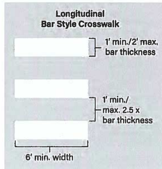
Figure 6-1 Crosswalk Dimensions
