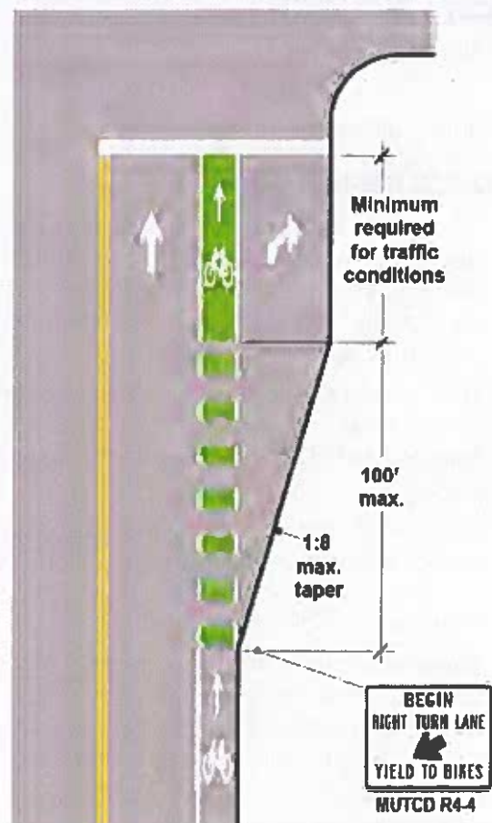
Figure 5-18 Bike Pocket
