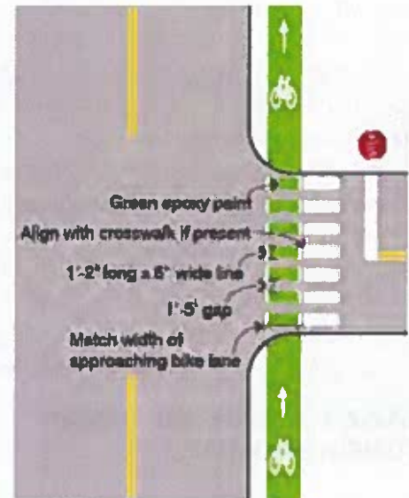
Figure 5-21 Green markings
