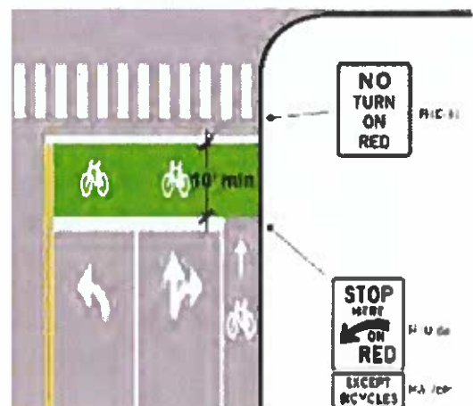
Figure 5-19 Bike Box
