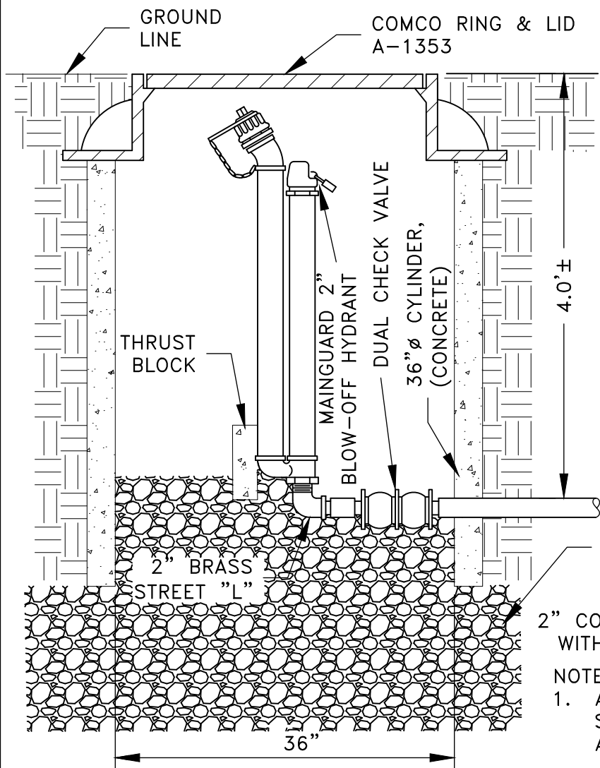
KUPFERLE MAINGUARD NO. 78 BLOW-OFF HYDRANT
