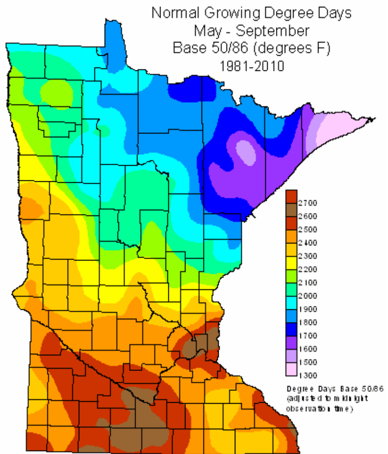
Figure 4-4: Growing Degree Days
