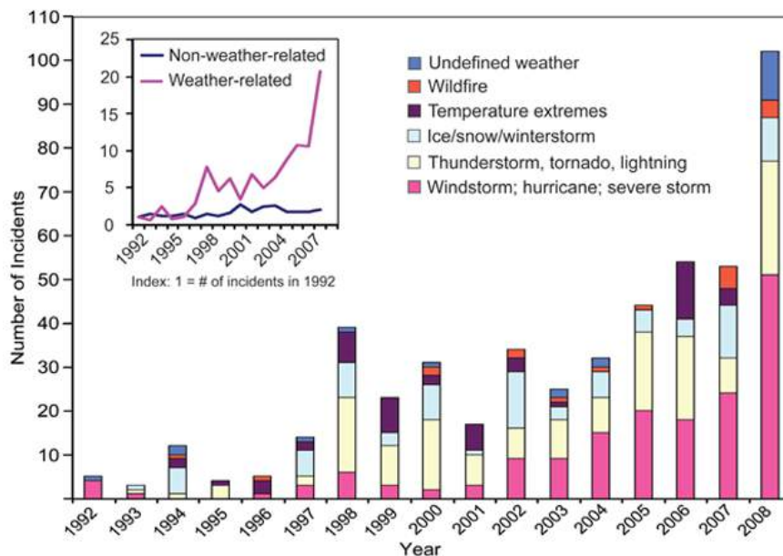
Figure 6-47: Significant U.S. Electrical Grid Disturbances, 1992-2011
