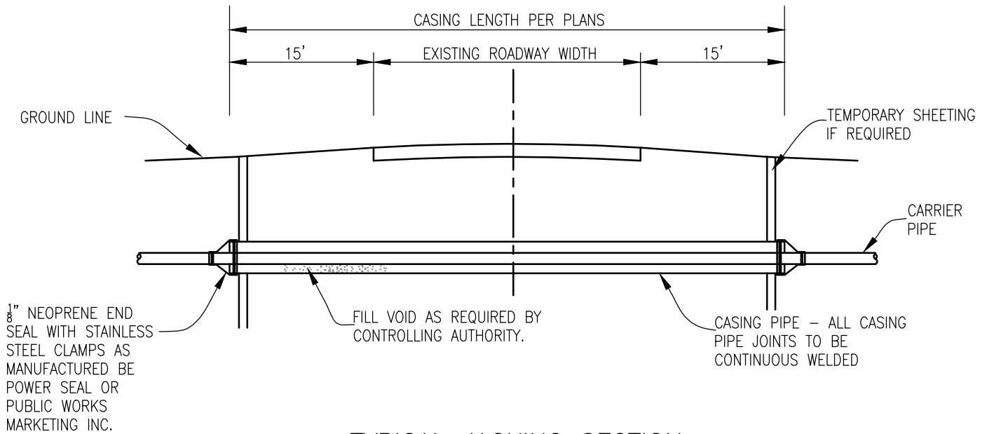
TYPICAL JACKING SECTION NO SCALE
