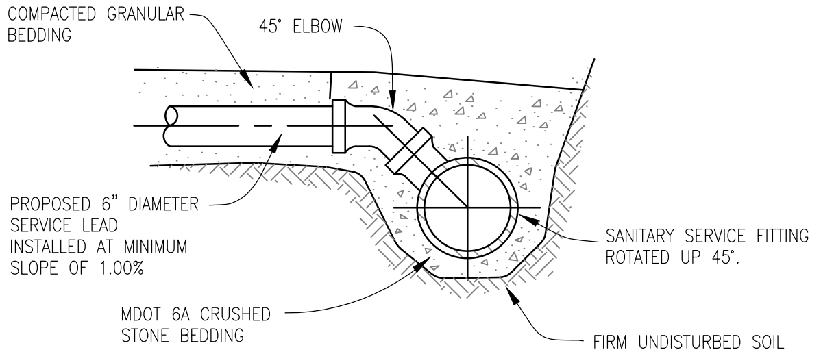
HORIZONTAL CONNECTION
