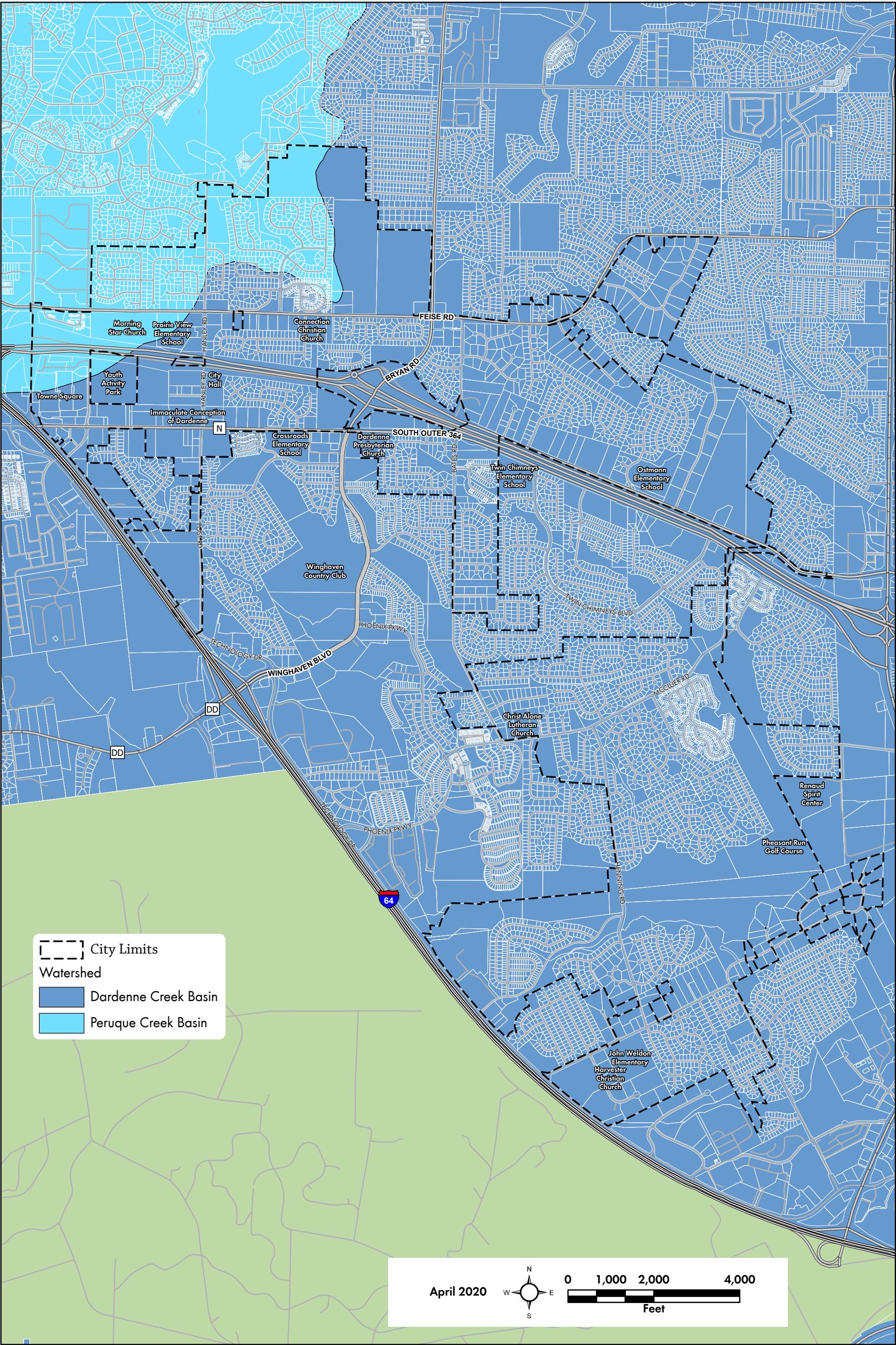
Figure 11 - Watersheds
